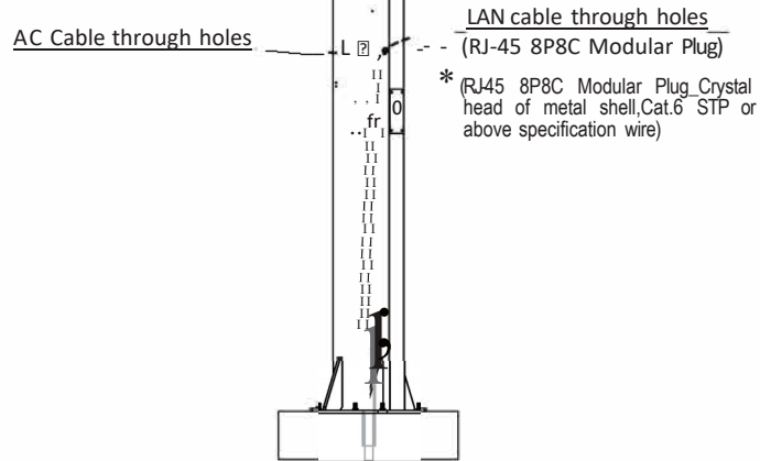
Fig. 8 Cable through holes
